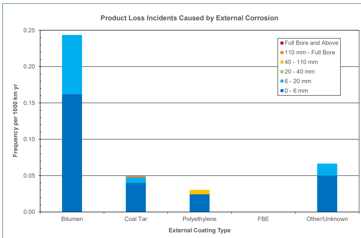
Figure 4.15: External Corrosion Product Loss Frequency by External Coating and Equivalent Hole Size
