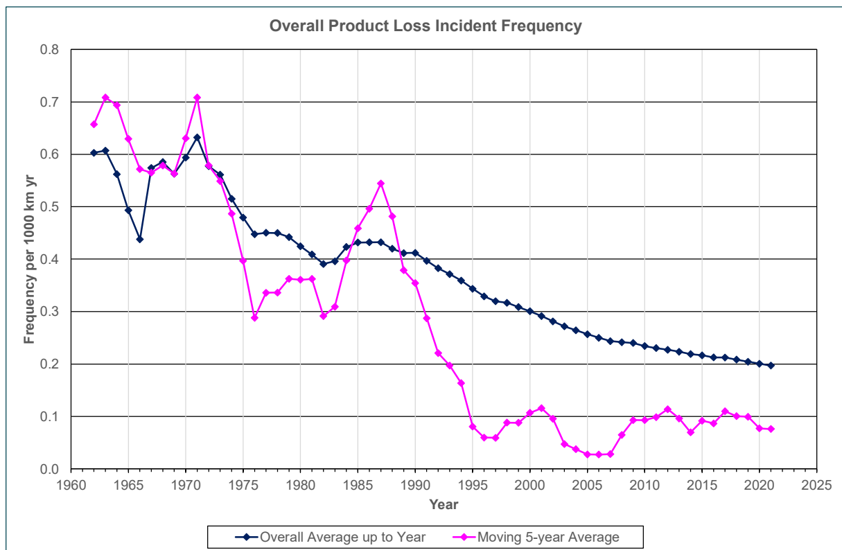
Figure 4.3: Development of overall and 5-year Incident Frequency
