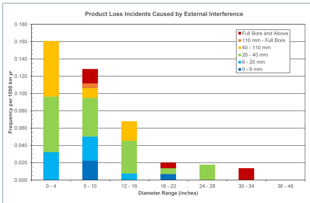
Figure 4.10: External Interference Product Loss Frequency by Diameter and Equivalent Hole Size
