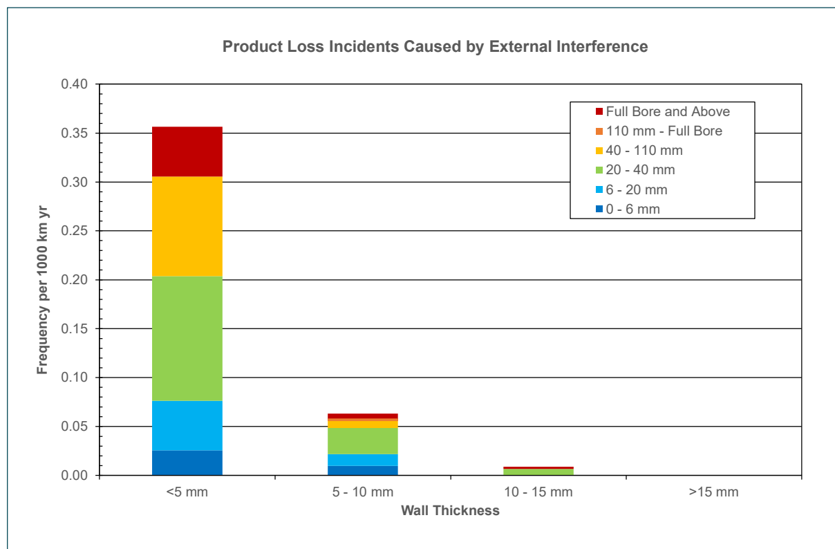
Figure 4.11: External Interference Product Loss Frequency by Wall Thickness and Equivalent Hole Size
