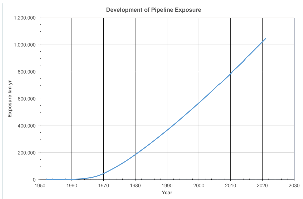
Figure 3.1: Pipeline Operating Exposure from 1952 to 2021
