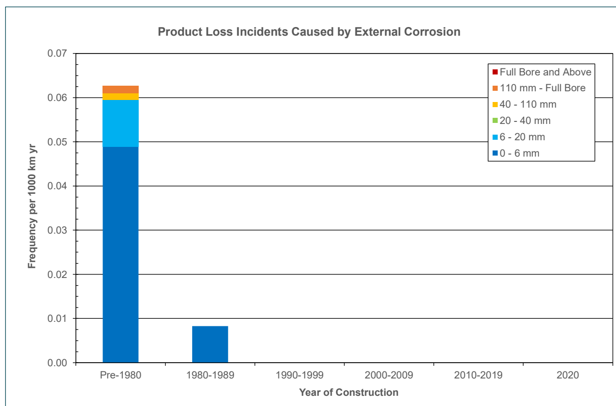
Figure 4.14: External Corrosion Product Loss Frequency by Year of Construction and Equivalent Hole Size
