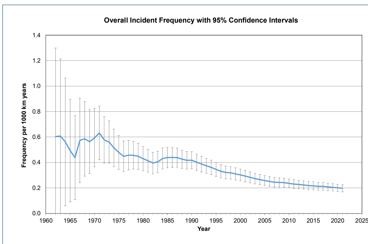
Figure 4.4: Overall Incident Frequency with 95% Confidence Intervals
