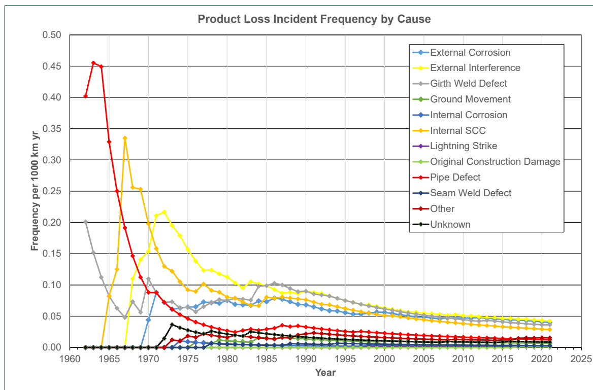
Figure 4.6: Product Loss Incident Frequency by Cause
