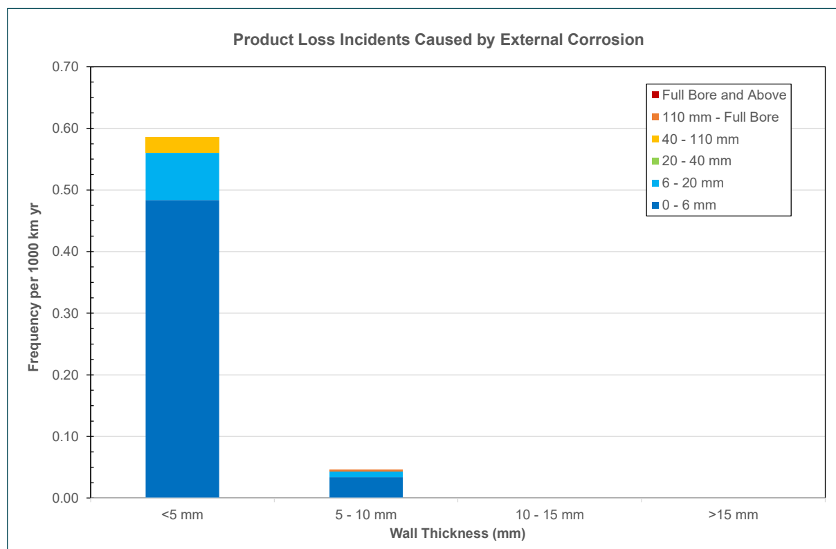
Figure 4.13: External Corrosion Product Loss Frequency by Wall Thickness and Equivalent Hole Size
