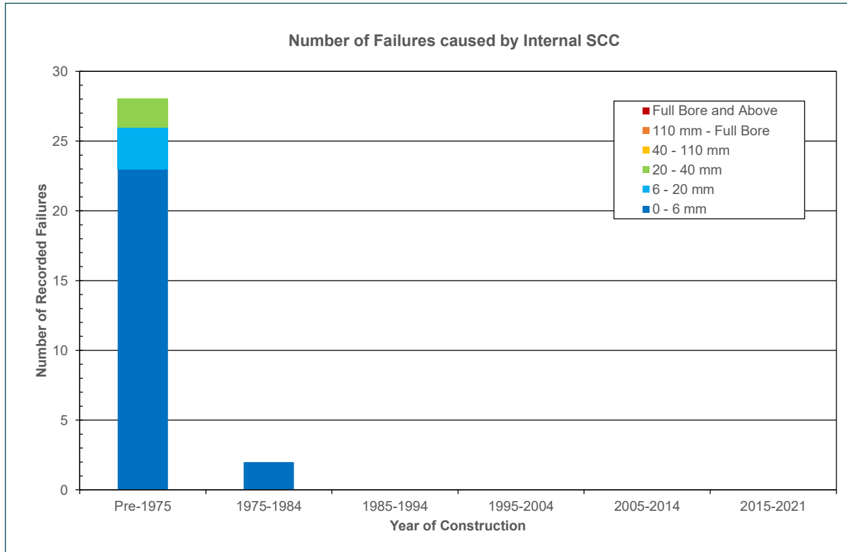
Figure 4.16: Internal SCC Product Loss Incidents by Year of Construction and Equivalent Hole Diameter
