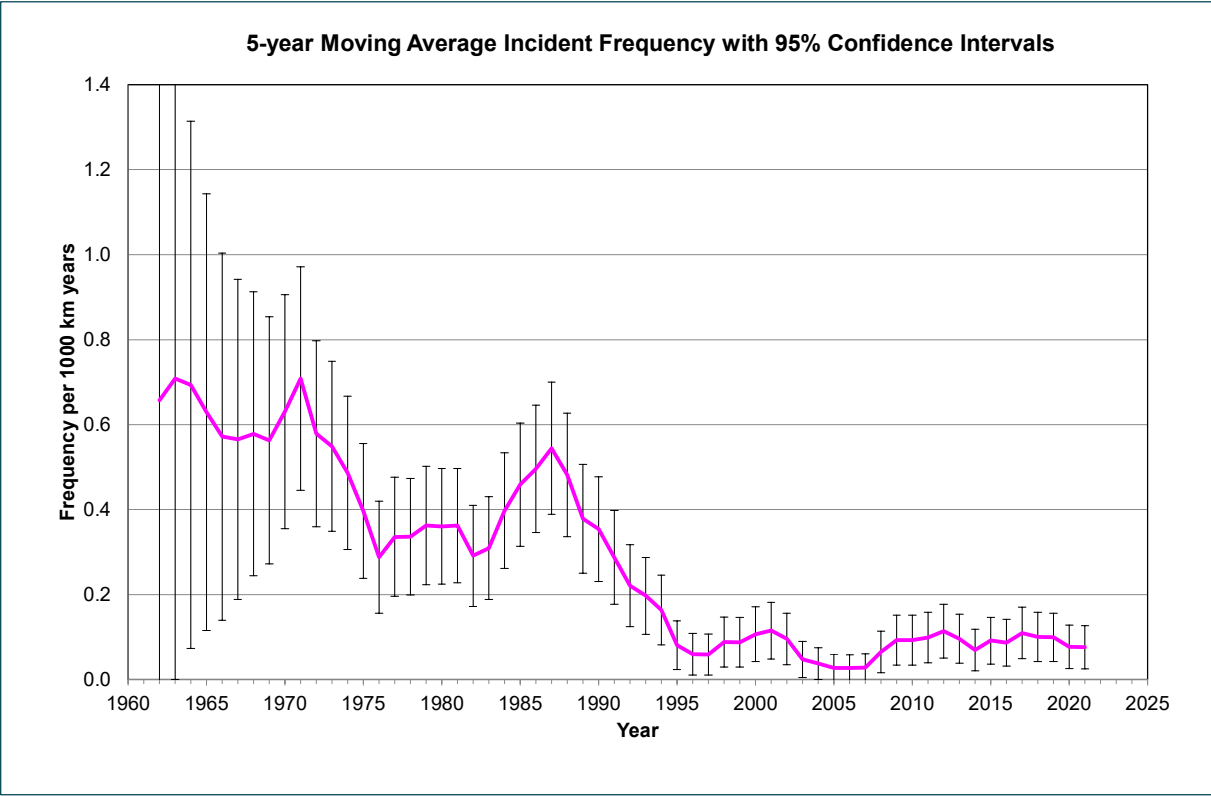
Figure 4.5: 5-year Incident Frequency with 95% Confidence Intervals
