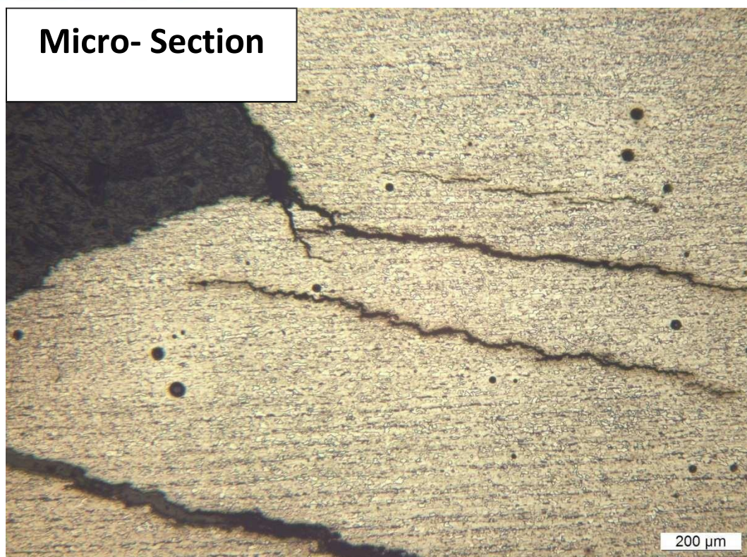
Figure 7 Circumferential SCC failure
