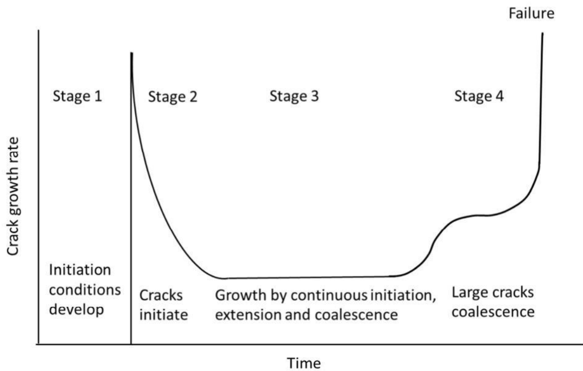
Figure 8 Bathtub Model Life Cycle of SCC growth in pipelines (Parkins, 1987)
